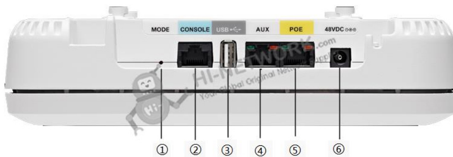
Figure 3 shows AIR-AP1852I Ports and Connections.
